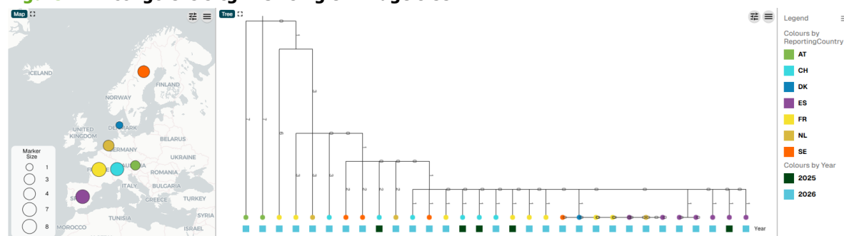
Figure 1. D. congolensis cgMLST single-linkage tree
